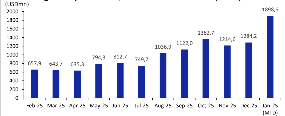
JCI Average Daily Turnover, Feb 2025 – Jan 2026 (MTD)
