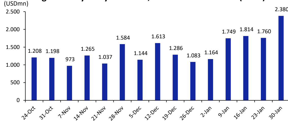
JCI Average Weekly Daily Turnover, Oct 2025 – Jan 2026 (MTD)
