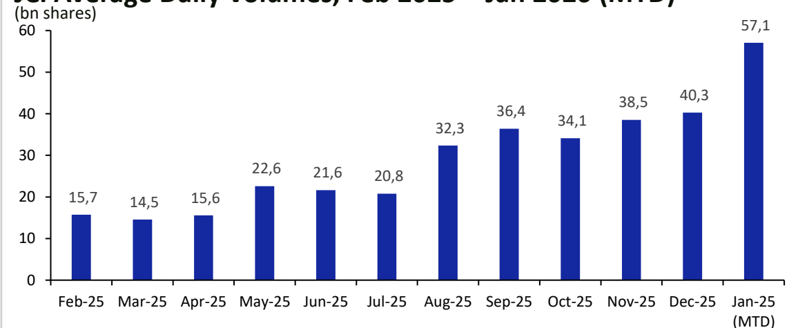
JCI Average Daily Volumes, Feb 2025 – Jan 2026 (MTD)
