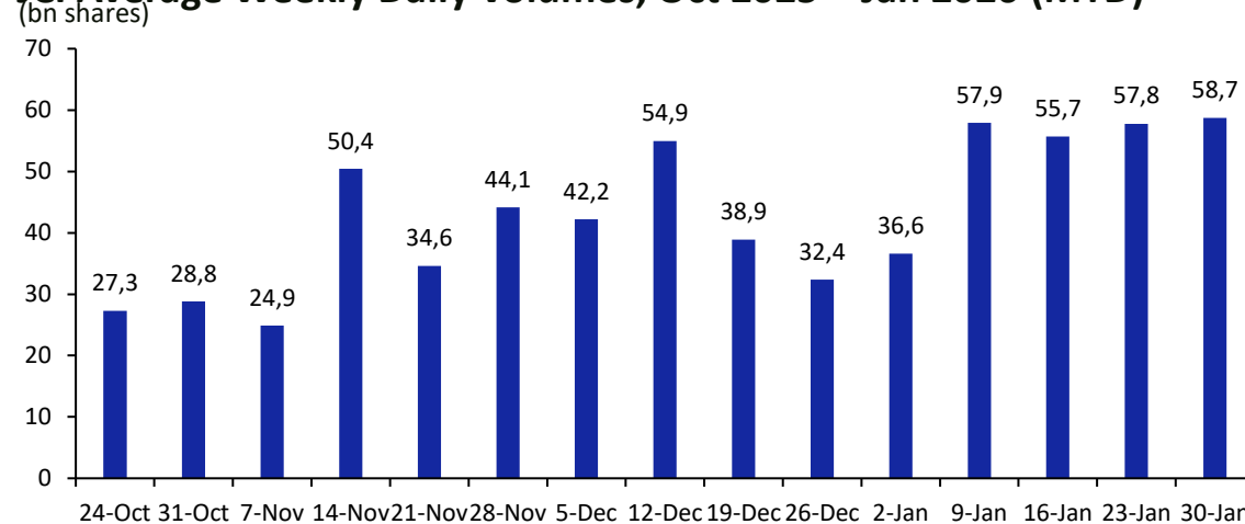
JCI Average Weekly Daily Volumes, Oct 2025 – Jan 2026 (MTD)
